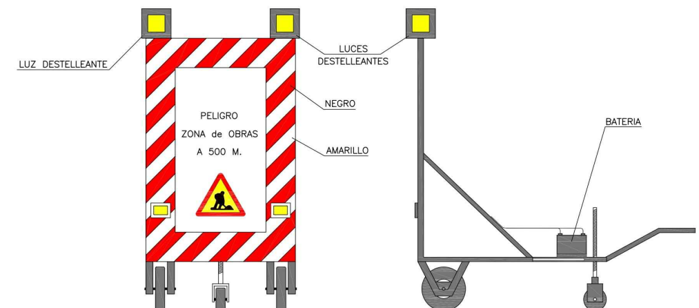
VISTA FRONTAL
