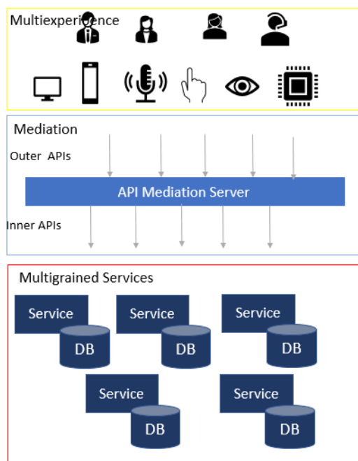
Mesh App and Service Architecture
